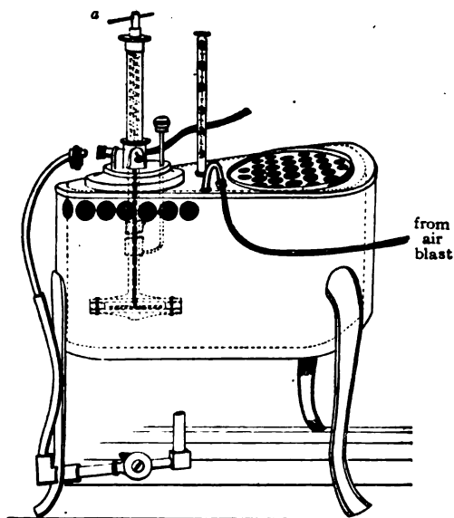
FIG. 155.—Hearson's water-bath.
